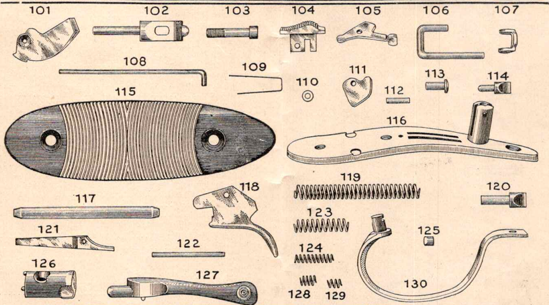
PART PRICES FOR LEFEVER GUNS NUMBERED OVER 100,000
